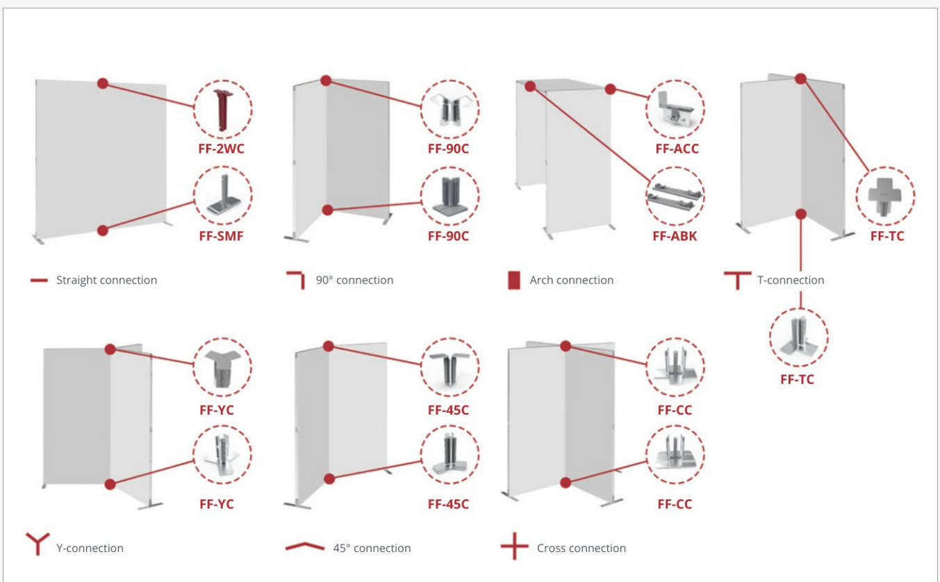
Y Shape Connector Kit (FF-YC)
